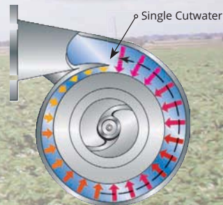
Single Volute
