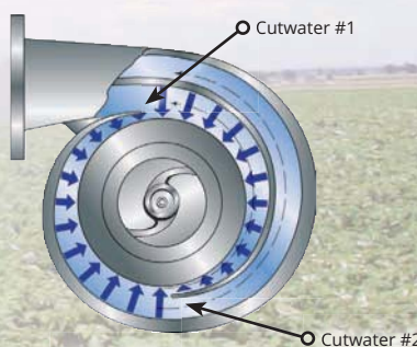
Double Volute
