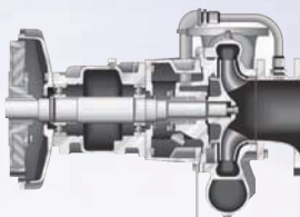
VM/VC/VF Close Coupled Coupled Frame Mount
